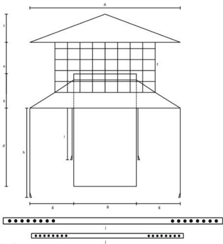
Pot Hanging Cowl - measurements
