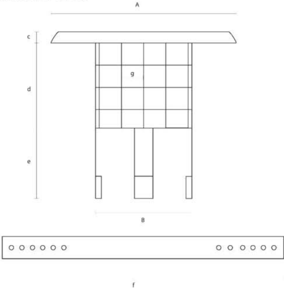
Anti-Bird/Anti Rain Cowl - diagram
